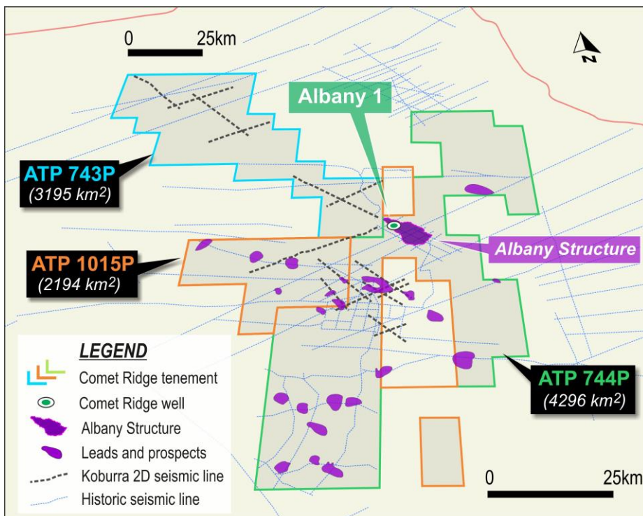
Figure 1 – Regional map of the Galilee Permits, showing the Kobarra 2D seismic lines
