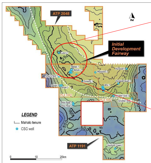
Figure 2 – Coal seam gas fairway running up from the Mahalo Gas Project into Mahalo North.
